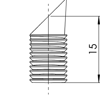
Fixi 45° Keyhole installation guide:
